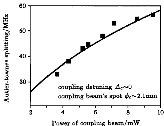
Fig.4. The frequency splitting of the Autler-Townes doublet in coupling beam's transmission for F_g=4-F_e=3 transition versus power of coupling beam. The solid squares are experimental data. Probe beam is kept at 35\mu\text{W} . Diameters of beam spots are approximately 1.5mm for probe beam and \sim 2.1\text{mm} for coupling beam in the caesium cell region. The solid curve is the theoretical result.
