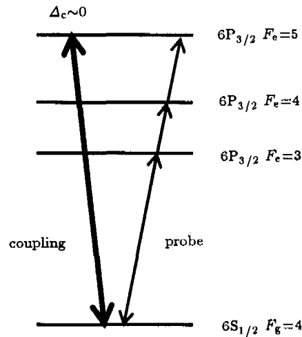
Fig.1. The relevant hyperfine levels of caesium atoms. The coupling laser is locked to 6S_{1/2} F_g=4-6P_{3/2} F_e=5 cycling transition (detuning to the cycling transition \Delta_c \sim 0 ), while the probe laser is scanned across the whole 6S_{1/2} F_g=4-6P_{3/2} F_e=3, 4, 5 three transitions.
